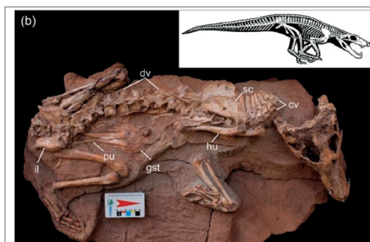
FIGURE 1 (a) Location of Bauru Basin within South America and its geological map. The Caiuá sequence is homogenized in gray, whereas stratigraphic units belonging the Bauru Group are highlighted in color. The specimen was collected in the vicinities of Fernandópolis-SP municipality, marked in white. (b) IFSP-VTP/PALEO-0003 specimen in dorsolateral view. All but the caudal series is preserved as shown by the skeletal reconstruction on the top right corner (by Felipe Alves Elias). cv, cervical vertebrae; dv, dorsal vertebrae; gst, gastralia; hu, humerus; il, ilium; pu, pubis. Scale bar in (b) = 1 m.
